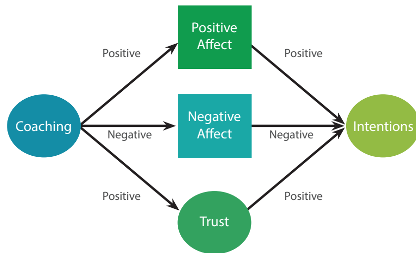
Figure 1 – Hypothesized Pathway Model
